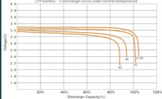
常溫下LYP類電池的放電特性曲線 LFP battery's discharge curve under normal temperature
